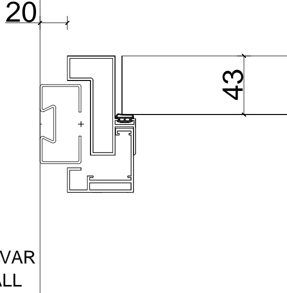
WOODEN DOOR WALL CONNECTION DETAIL AHŞAP KAPI DUVAR BAĞLANTI DETAYI
