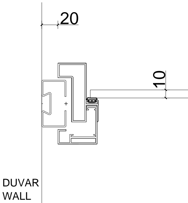
GLASS DOOR WALL CONNECTION DETAIL CAM KAPI DUVAR BAĞLANTI DETAYI
